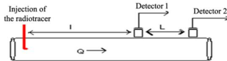
Figure 3.10: Schematic Arrangement of Transient Time methodology.
