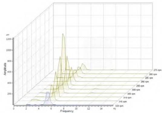
Figure 3.2: Test result to identify the translation mode in X direction. (Frequency sweep tests)
