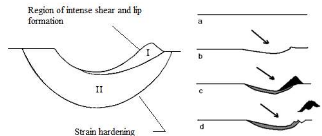
Figure 3.23: crater formed by dynamic impact of particles. Extracted from (Shewmon and Sundararajan, 1983).
