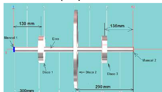
Figure 3.4: Rotor Model
