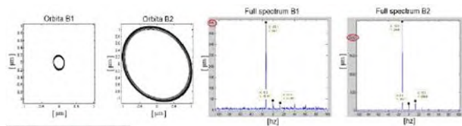
Figure 3.17: Orbit and Full spectrum for static unbalance test B1 and B2.
