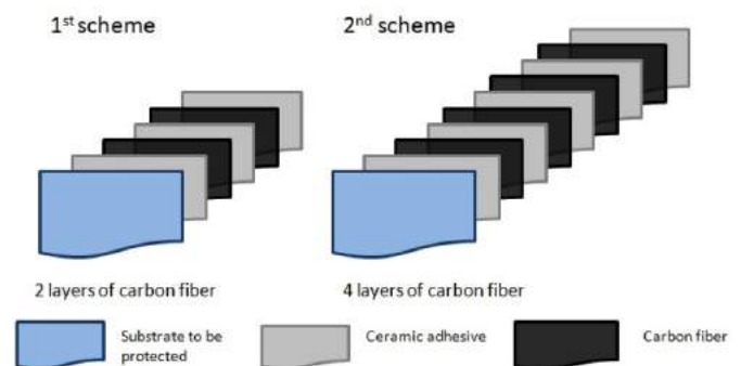
Figure 3.24: Schematic assembly of the two proposed coating schemes for the water wall piping of thermoelectric boilers.
