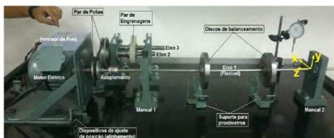
Figure 3.16: Experimental Rig.
