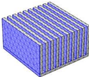
Figure 3.20: Longitudinal convecting-radiating copper fin
