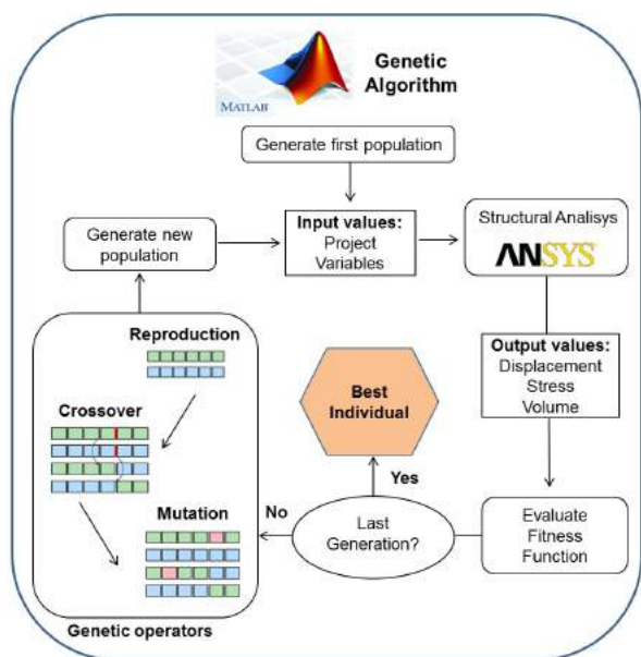
Figure 3.13: Genetic algorithm optimization interfacing MATLAB and ANSYS
