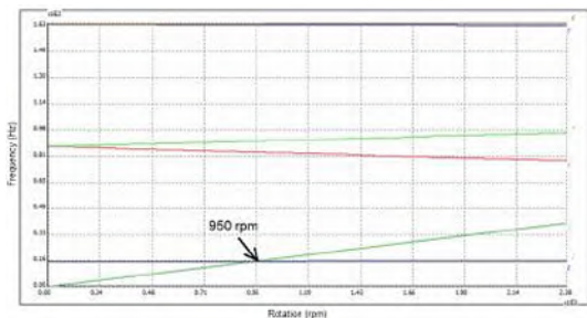
Figure 3.5: Campbell Diagram
