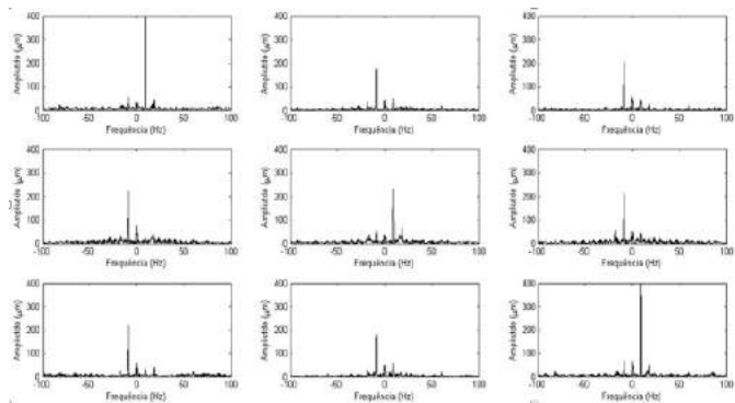
Figure 3.7: Tests results of first configuration in 550 Rpm (Full Spectrum Matrix)
