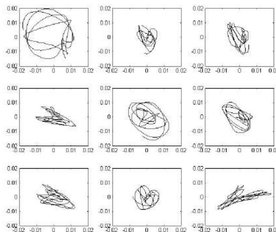
Figure 3.8: Matrix Orbits-Tests Configuration1-550Rpm
