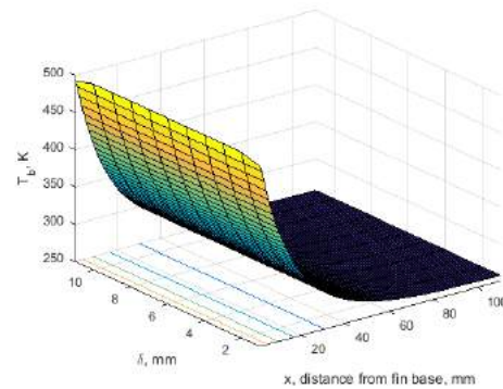
Figure 3.22: Temperature profile for a longitudinal convecting-radiating copper fins with mutual irradiation between radiator elements
