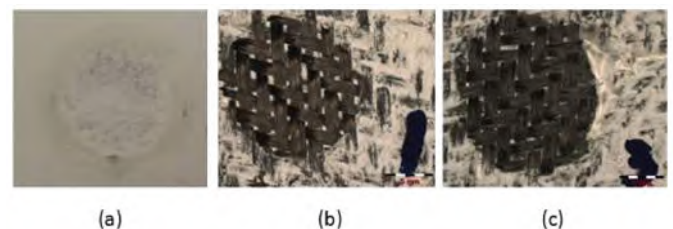
Figure 3.25: Figure 2: (a) Aspects obtained from the adhesion test for the substrate with only the first layer of ceramic adhesive. The nature of the Cohesive B failure was observed. (b) Result of the first protection coating assembly scheme. Nature of the type C failure. (c) Result of the second protection coating assembly scheme. Nature of failure: type C.
