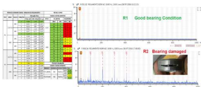
Figure 3.18: Results of bearing faults tests R1 and R2.
